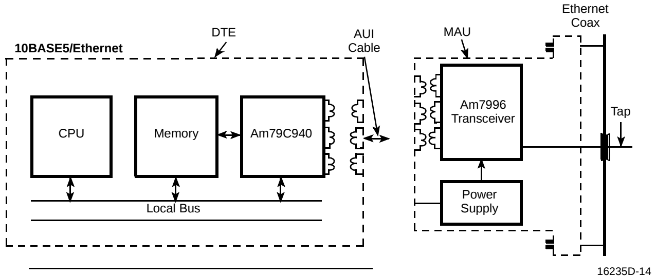
AUI-10BASE5/Ethernet Example
