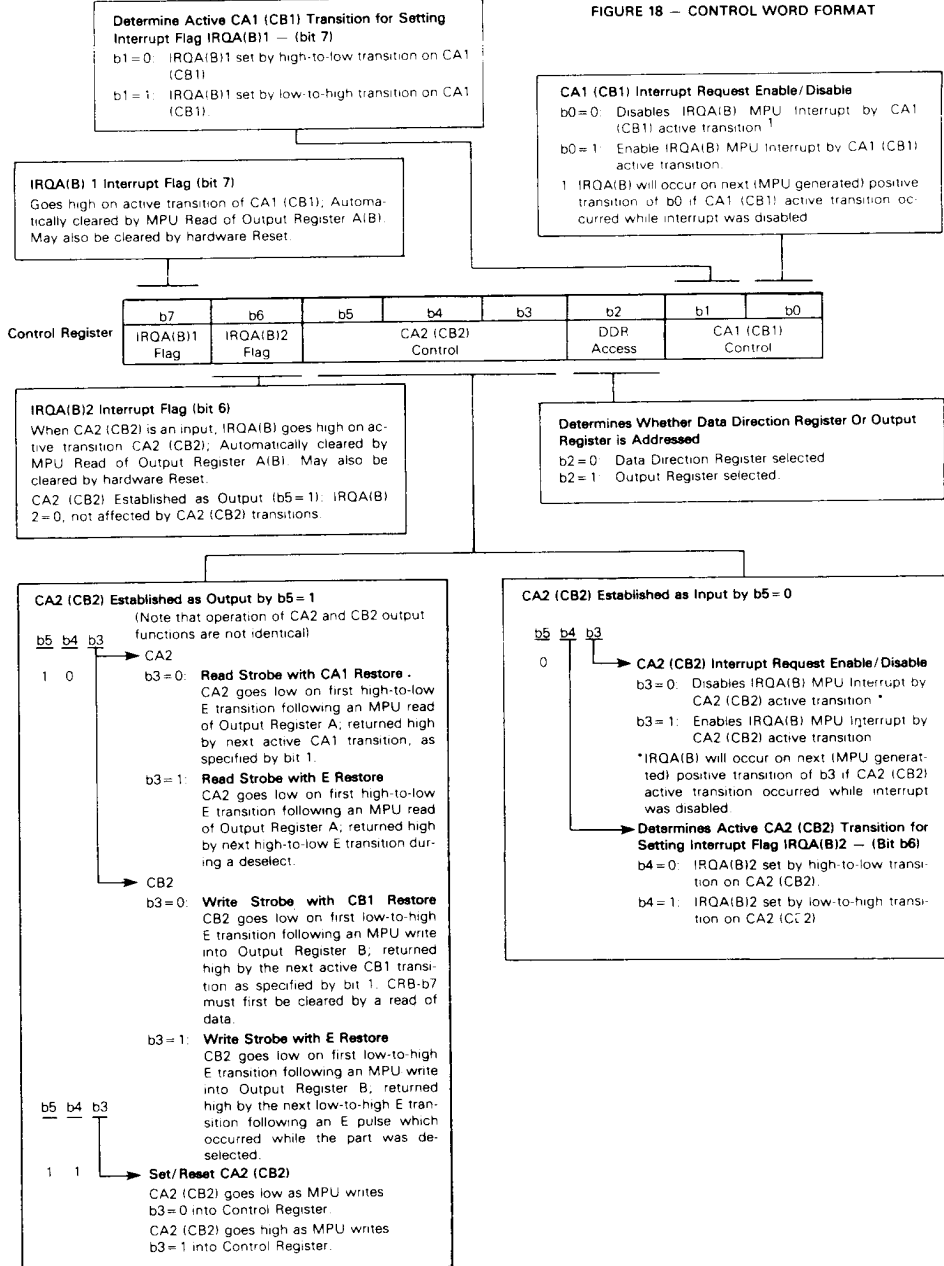
FIGURE 18 — CONTROL WORD FORMAT
