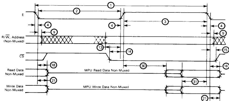
FIGURE 1 — BUS TIMING
