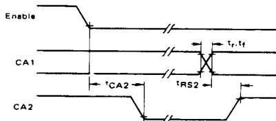
FIGURE 8 — CA2 DELAY TIME (Read Mode; CRA-5 = CRA3 = 1, CRA-4 = 0)
