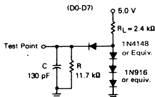
FIGURE 2 — BUS TIMING TEST LOADS
