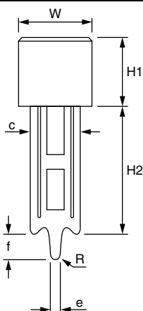
TERMINAL STYLE 1 (SINGLE PIN)
