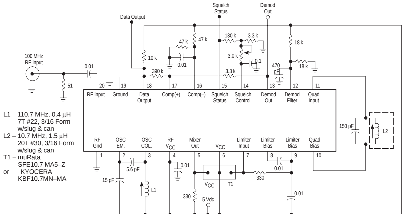
Figure 2. Test Circuit
