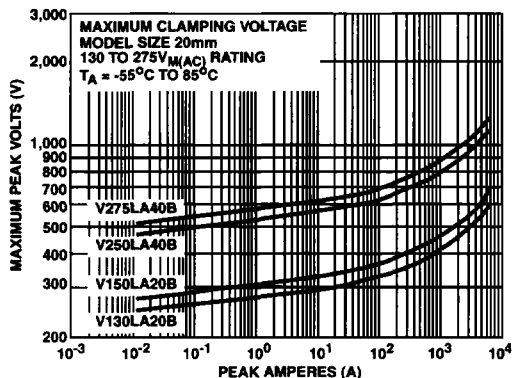
FIGURE 11. CLAMPING VOLTAGE FOR V130LA20B - V275LA40B
