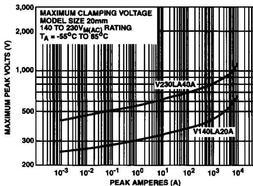
FIGURE 12. CLAMPING VOLTAGE FOR V140LA20A - V230LA40A
