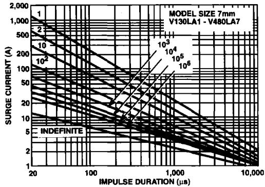
FIGURE 14. SURGE CURRENT RATING CURVES FOR V130LA1 - V480LA7
