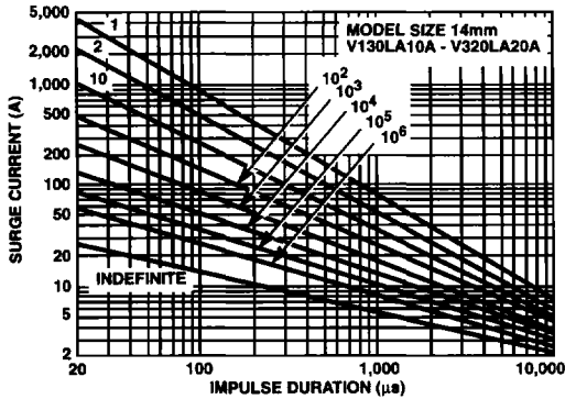
FIGURE 16. SURGE CURRENT RATING CURVES FOR V130LA10A - V320LA20A
