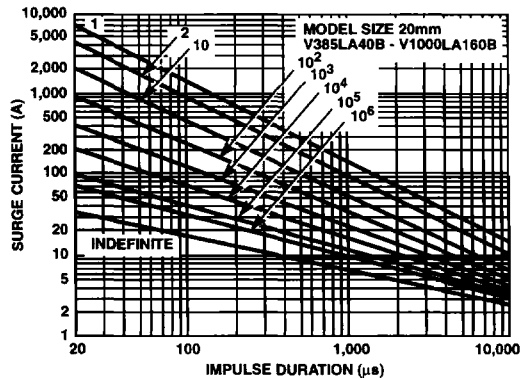
FIGURE 19. SURGE CURRENT RATING CURVES FOR V385LA40B - V1000LA160B
