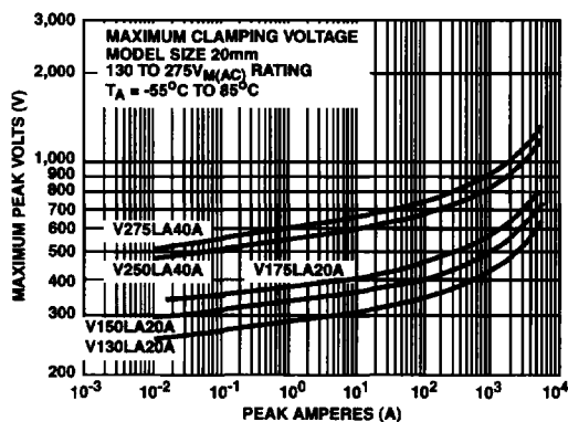
FIGURE 10. CLAMPING VOLTAGE FOR V130LA20A - V275LA40A
