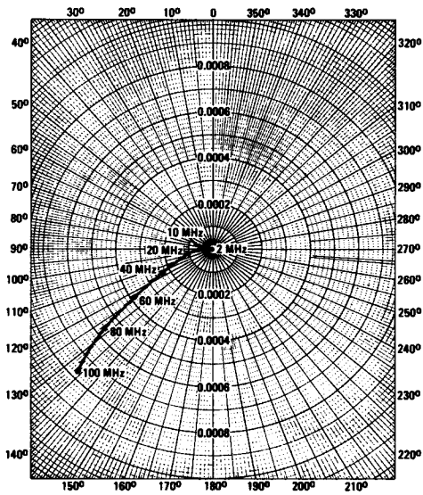
FIGURE 23 — s_{12} , REVERSE TRANSMISSION COEFFICIENT (FEEDBACK)
