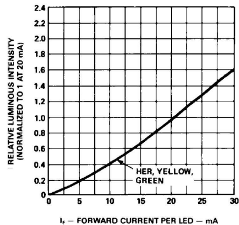
Figure 10. Relative Luminous Intensity vs. DC Forward Current.
