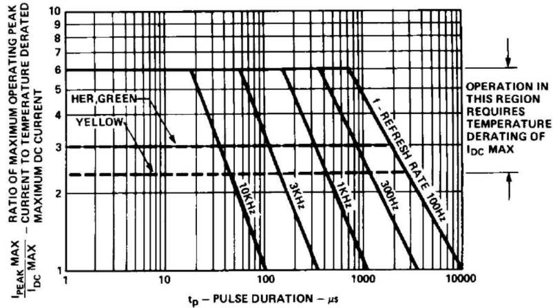
Figure 6. Maximum Allowed Peak Current vs. Pulse Duration.
