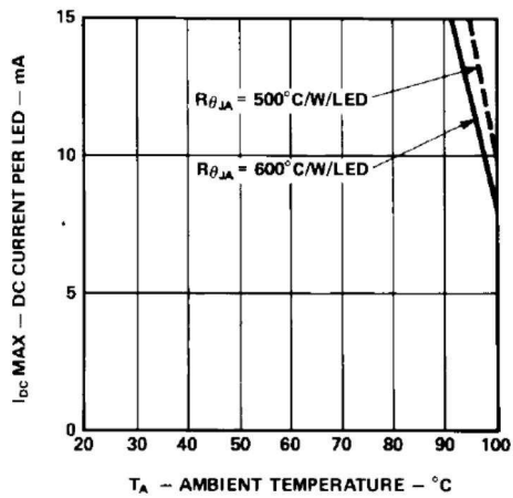
Figure 2. Maximum Allowed DC Current per LED vs. Ambient Temperature, T_{J MAX} = 110^\circ\text{C} .
