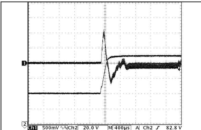
Figure 15: Output voltage response to step-change in input voltage (50V to 100V in 200 \mu s). Load cap: 470 \mu F, 15 mW ESR tantalum capacitor. Ch 1: Vout (500mV/div), Ch 2: Vin (20V/div), at zero load current.
