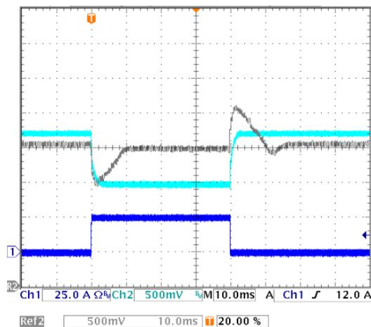
Figure D: Output voltage response to full load step change in output current (Ch2), compared to a fully regulated QEA model (Ref2). 12mF output capacitance.
