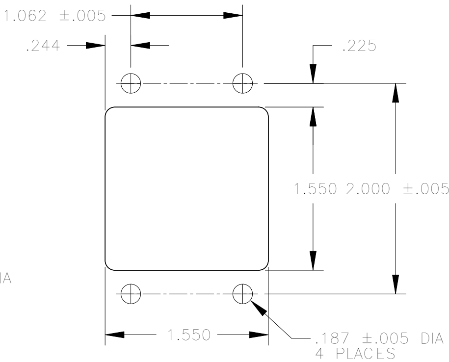
SUGGESTED MOUNTING HOLE LAYOUT FOR BRACKET MOUNTING
