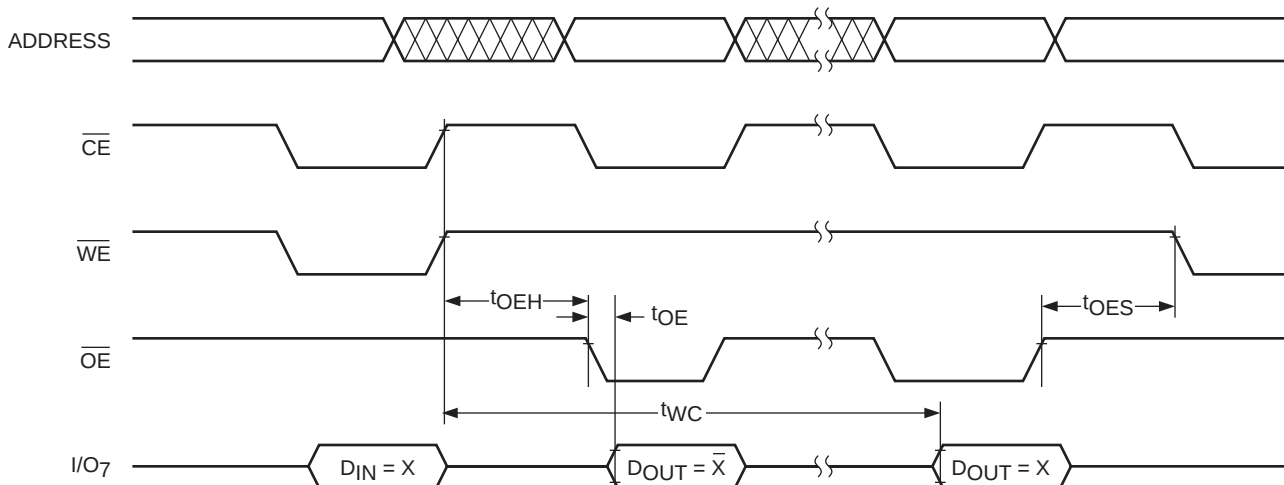
Figure 6. DATA Polling
