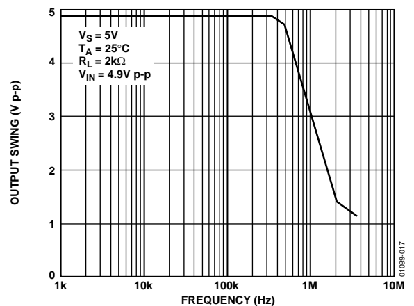
Figure 17. Closed-Loop Output Voltage Swing vs. Frequency
