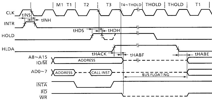
Figure 12.5 Interrupt and Hold Timing
