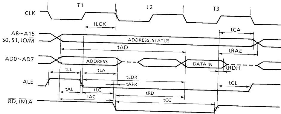
Figure 12.2 Read Operation
