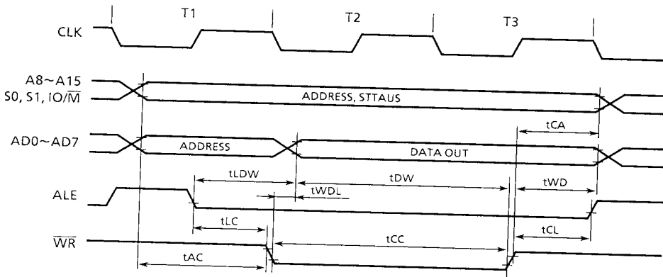
Figure 12.3 Write Operation
