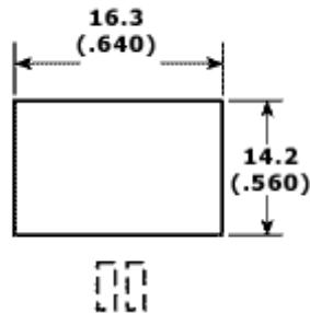
Recommended Cu Heat Spreader Drain Pad
