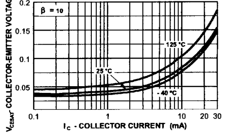
Collector-Emitter Saturation Voltage vs Collector Current
