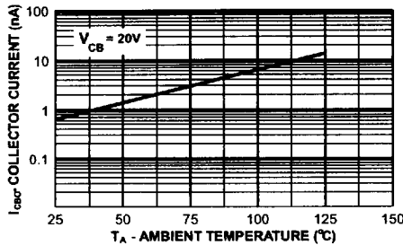
Collector-Cutoff Current vs Ambient Temperature
