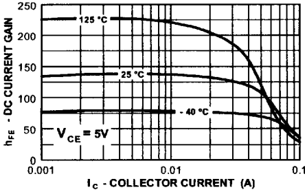
DC Current Gain vs Collector Current
