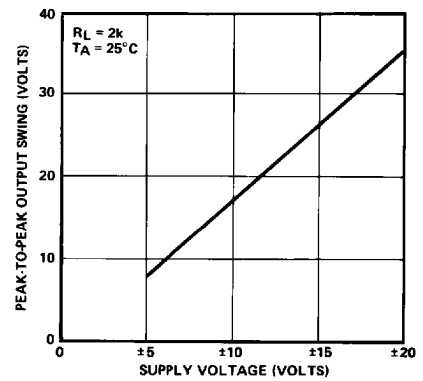
OUTPUT VOLTAGE SWING vs SUPPLY VOLTAGE
