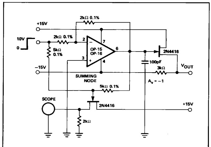
SETTLING-TIME TEST CIRCUIT — OP-15/OP-16
