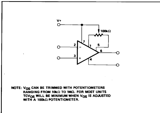
INPUT OFFSET VOLTAGE NULLING
