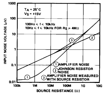
VOLTAGE NOISE vs SOURCE RESISTANCE
