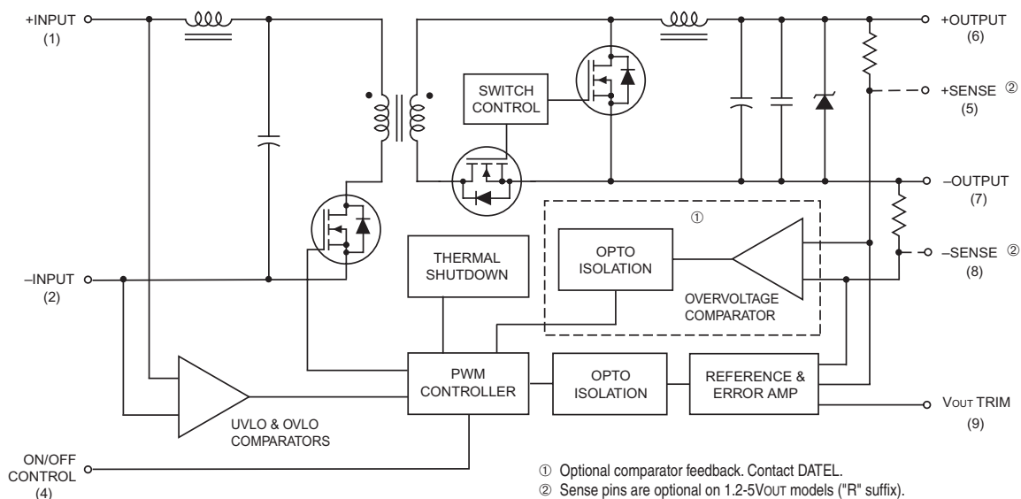
Figure 1. Simplified Schematic
