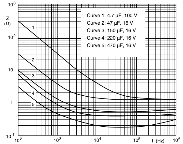
Case \varnothing D x L = 6.5 x 18 mm to 10 x 25 mm T_{\text{amb}} = 20 °C
