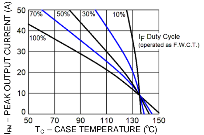
FIGURE 2 Peak Output Current vs. Case Temperature
