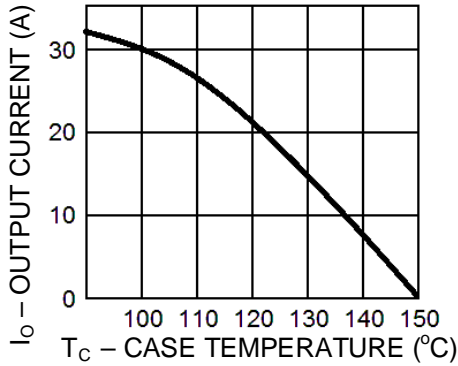
FIGURE 1 Output Current vs. Case Temperature
