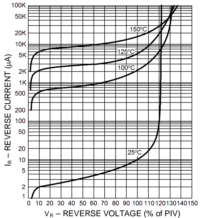
FIGURE 4 Typical Reverse Current vs. Reverse Voltage
