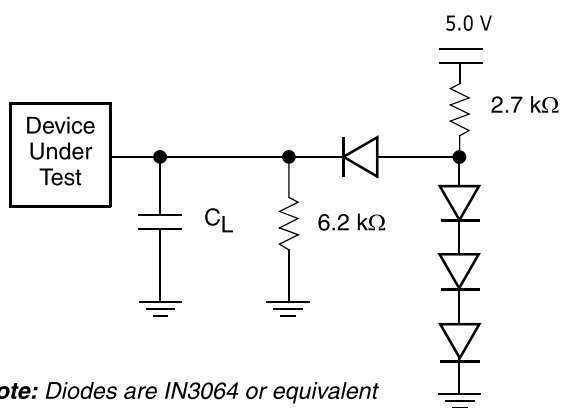
Figure 7. Test Setup
