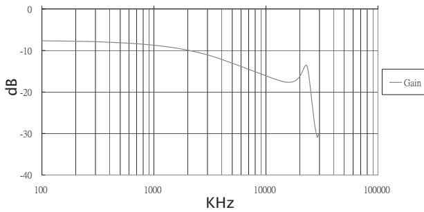
COMMON MODE
