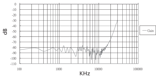
DIFFERENTIAL MODE
