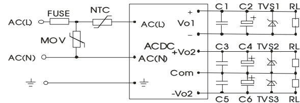
Fig. 4: LH10-10Cxx (Triple Output) series typical circuit diagram
