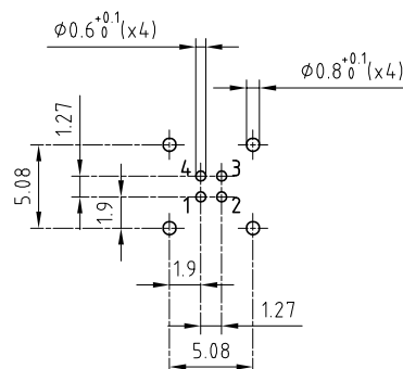
A-A cross-section (PCB drilling pattern)
