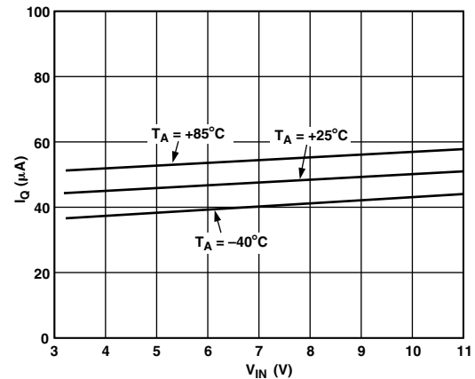
Figure 7. Typical Supply Current over Temperature
