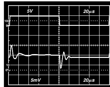
Figure 14. Load Transient Response (0 mA to 5 mA Load)
