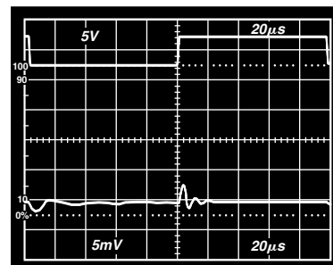
Figure 15. Load Transient Response (0 mA to -1 mA Load)
