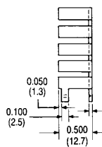
287 SERIES Wave-Solderable Low-Cost Heat Sinks
