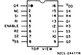
TOP VIEW 92CS-24477R1 CD4044B
