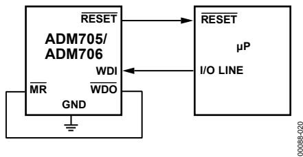
Figure 18. \overline{\text{RESET}} from \overline{\text{WDO}}
