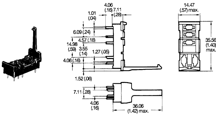
Terminal arrangement
