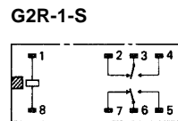
Terminal arrangement/Internal connections (Bottom view)
