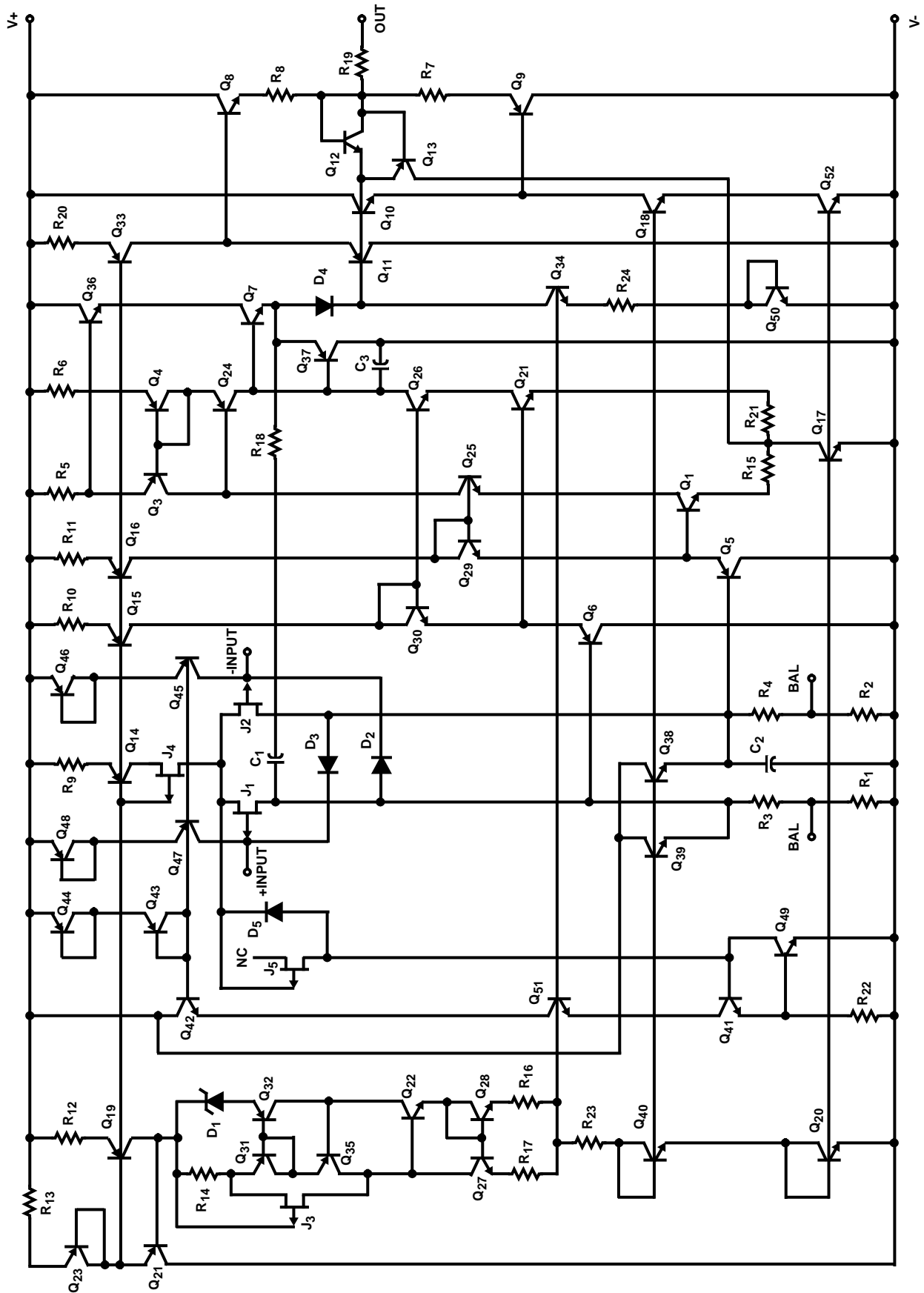
Schematic Diagram
