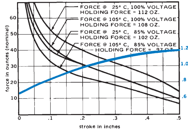
AC PULSE DUTY - 80VA
