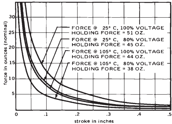
DC INTERMITTENT DUTY - 11.5 WATTS
