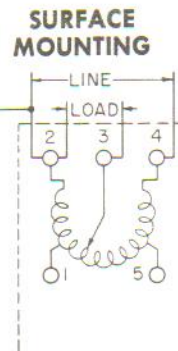
Figure 6. Recommended line-voltage connections
