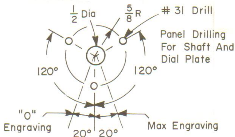
Figure 7. Mounting Dimensions
