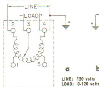
BACK-OF-PANEL MOUNTING
