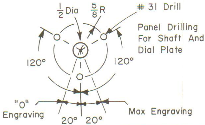
Figure 7. Mounting Dimensions (Cont.)
