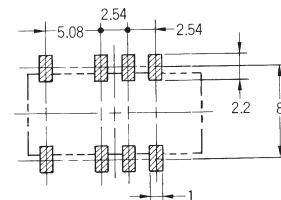
Footprint (Top View)
